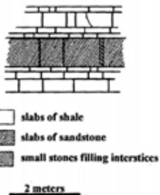
Sketch of elevation showing masonry on wall face v, Structure I at Kulli
